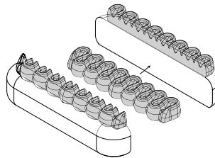
Base mould
